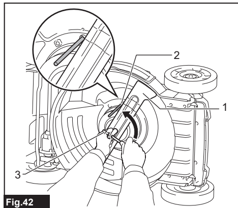
Fig.42 ► 1. Mower blade 2. Pin 3. Box wrench
